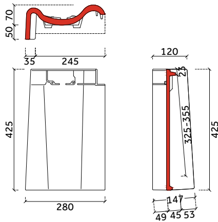
ondergevelpan links
