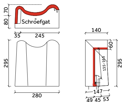
chaperongevelpan links 90°
