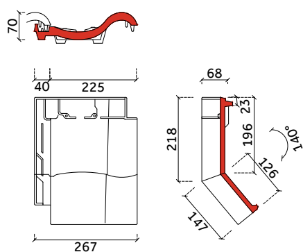
knikpan 140°
